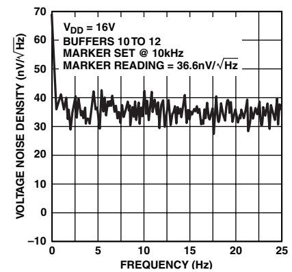
TPC 23. Voltage Noise Density vs. Frequency
