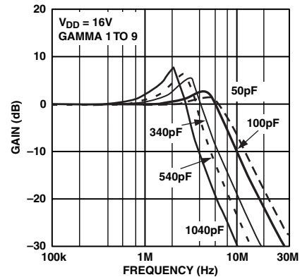
TPC 6. Frequency Response vs. Capacitive Loading
