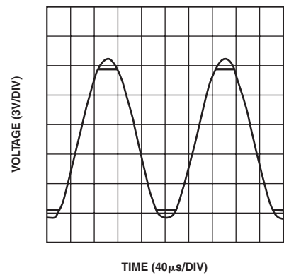
TPC 21. No Phase Reversal
