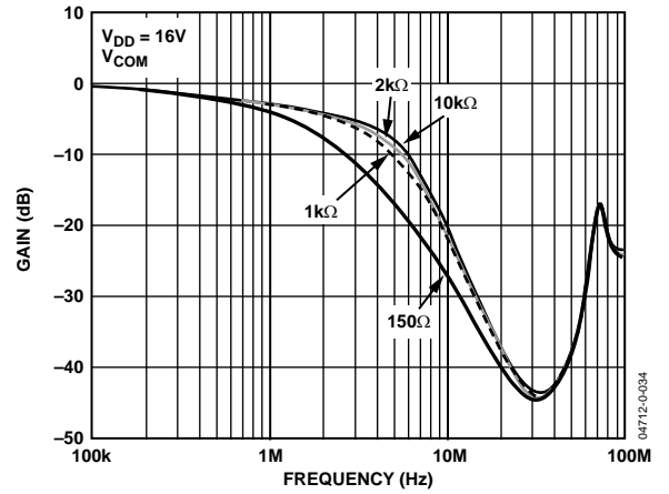
Figure 26. Frequency Response vs. Resistive Loading
