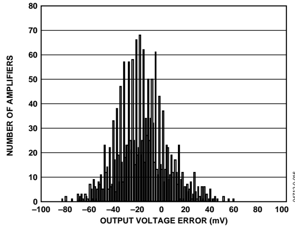
Figure 13. Output Voltage Error/Gamma 10 to 16
