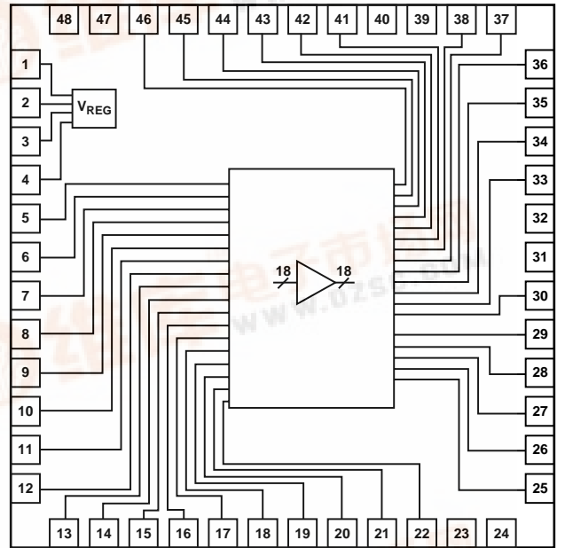
Figure 1. 48-Lead LQFP
