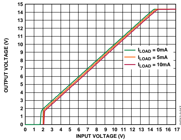
Figure 15. Dropout Characteristics
