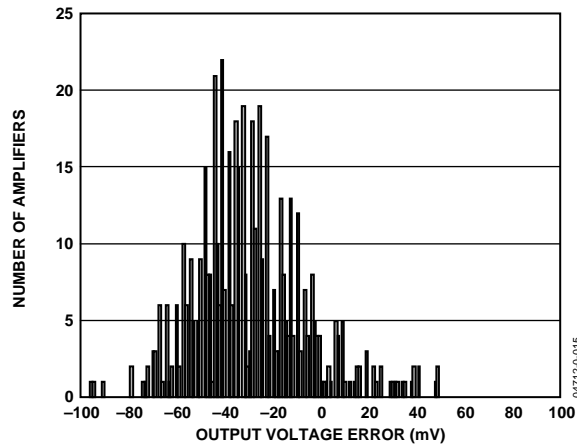
Figure 14. Output Voltage Error/Gamma 17 and 18
