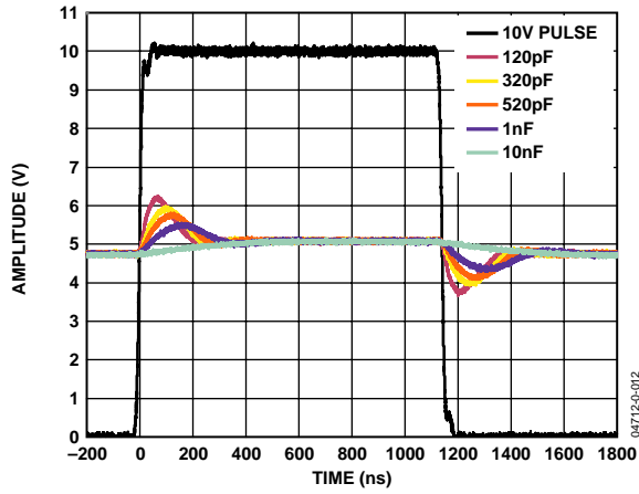
Figure 22. Transient Load Response vs. Capacitive Loading
