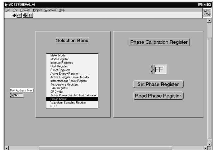
Figure 11—Writing to the PHCAL register to correct phase error
