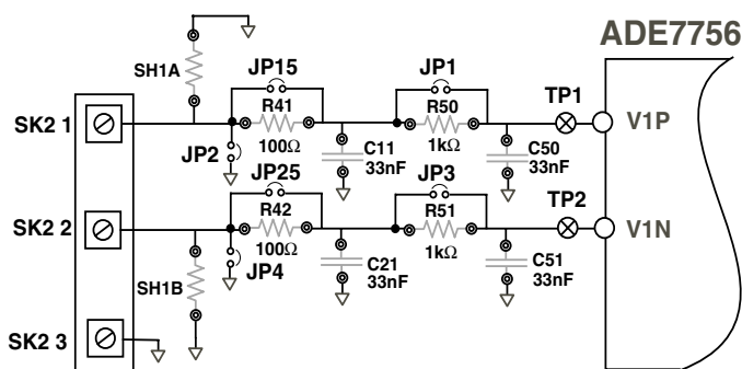
Figure 1 — Current Channel on the ADE7756 evaluation board
