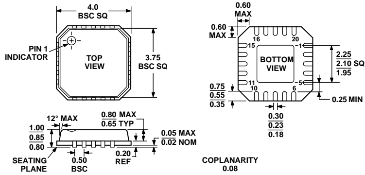
Figure 15. 20-Lead Frame Chip Scale Package [LFCSP] (CP-20)
