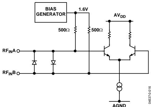
Figure 10. RF Input Stage
