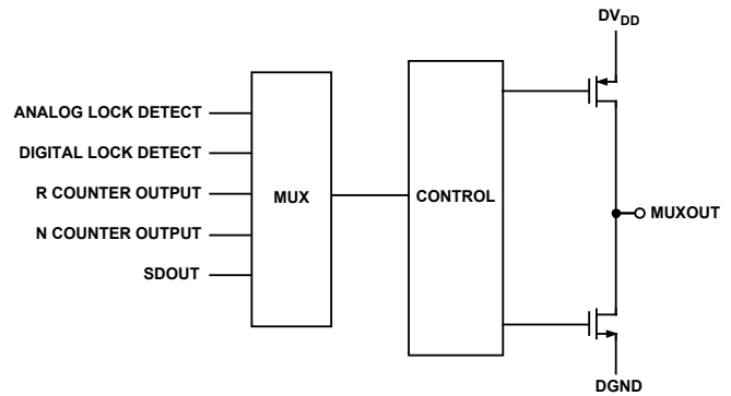
Figure 21. MUXOUT Circuit
