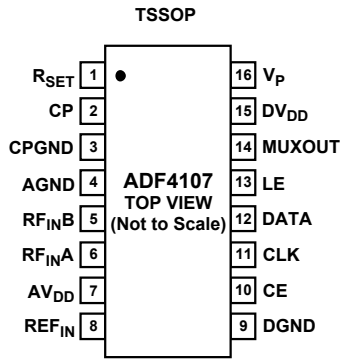
Figure 3. ADF4107 TSSOP (Top View)
