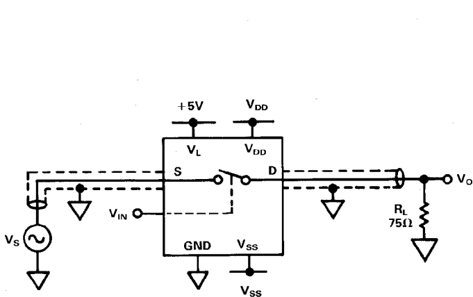
Test Circuit 5
