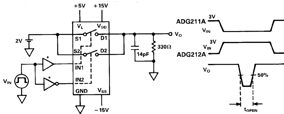
Test Circuit 1
