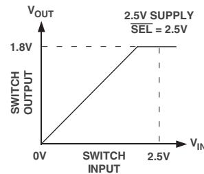
Figure 8. 2.5 V to 1.8 V Voltage Translation, \overline{SEL} = 2.5\text{ V}
