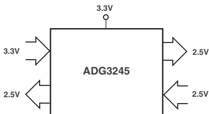
Figure 5. 3.3 V to 2.5 V Voltage Translation, \overline{SEL} = 3.3\text{ V}
