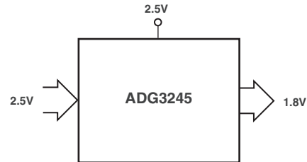
Figure 7. 2.5 V to 1.8 V Voltage Translation, \overline{SEL} = 2.5\text{ V}
