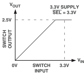
Figure 6. 3.3 V to 2.5 V Voltage Translation, \overline{SEL} = 3.3\text{ V}
