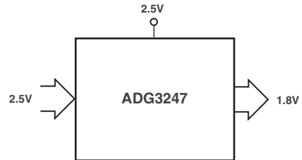
Figure 7. 2.5 V to 1.8 V Voltage Translation, \overline{SEL} = V_{CC}
