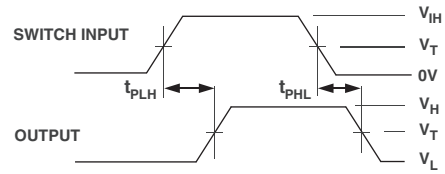
Figure 2. Propagation Delay
