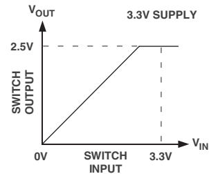
Figure 3. 3.3 V to 2.5 V Voltage Translation
