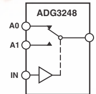
SWITCHES SHOWN FOR A LOGIC 0 INPUT
