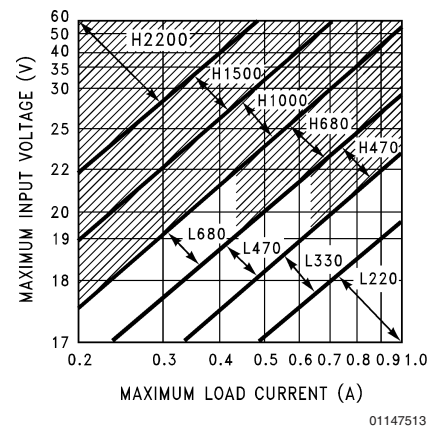
FIGURE 6. LM2575(HV)-15
