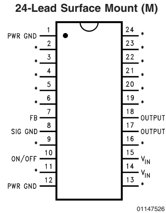
Top View LM2575M-XX or LM2575HVM-XX See NS Package Number M24B
