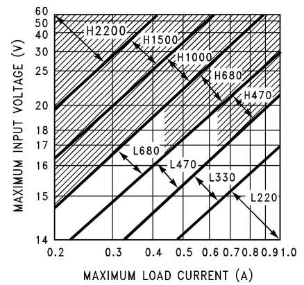
FIGURE 5. LM2575(HV)-12
