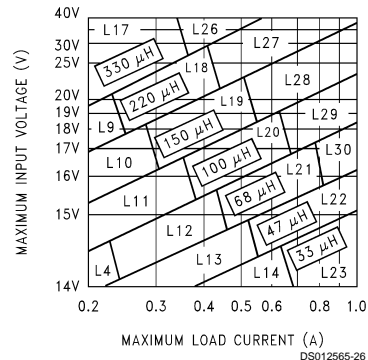
FIGURE 6. LM2595-12
