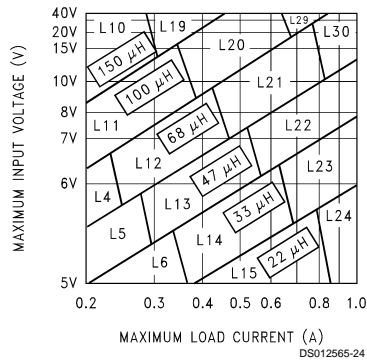
FIGURE 4. LM2595-3.3
