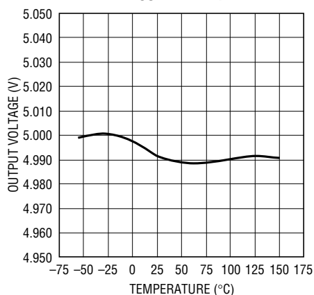
LT1575-5 V_{OUT} vs Temperature
