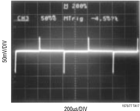
Transient Response to a 10A Load Step
