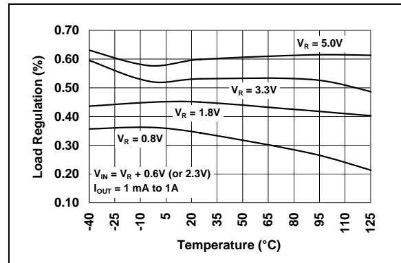
FIGURE 2-5: Load Regulation vs. Temperature.
