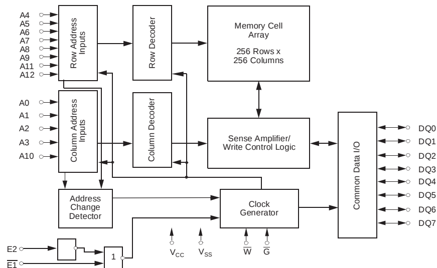
Block Diagram
