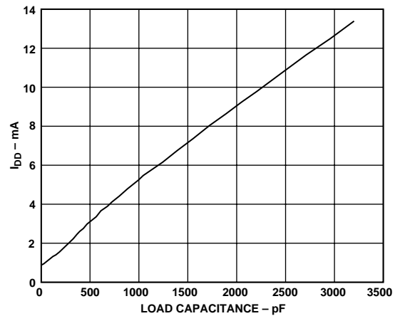
Figure 2. I DD vs. Load Capacitance @ 460 kbps
