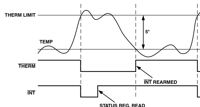
Figure 5. Operation of \overline{\text{THERM}} and \overline{\text{INT}} Signals
