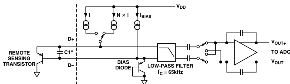
*CAPACITOR C1 IS OPTIONAL. IT SHOULD ONLY BE USED IN NOISY ENVIRONMENTS. C1 = 2.2nF TYPICAL, 3nF MAX.
