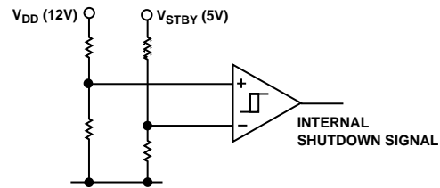
Figure 21. Standby Detection Circuit
