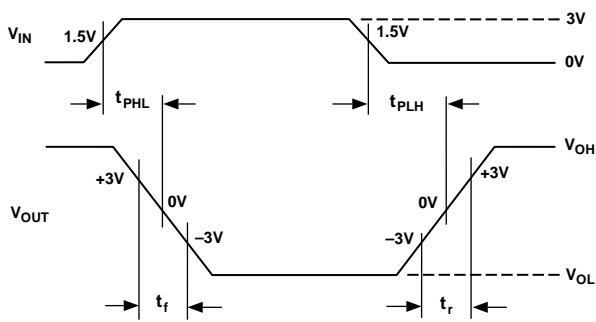
Figure 2. Driver Propagation Delay and Transition Time Waveforms
