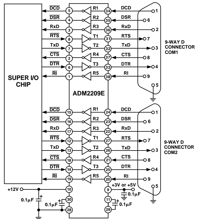
Figure 28. Typical Application for a Dual Serial Port
