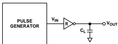
Figure 3. Test Circuit for Receiver Propagation Delay and Transition Time
