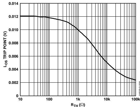
Figure 4. L_O5 Trip Point vs. Threshold Adjust Resistor
