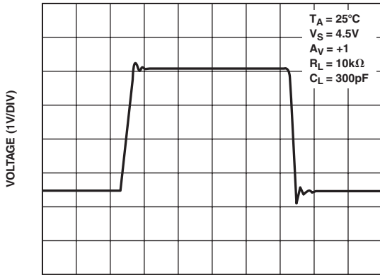
TIME (2µs/DIV)
