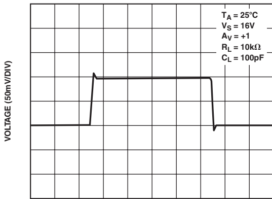
TIME (1µs/DIV)
