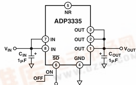
Figure 1. Typical Application Circuit
