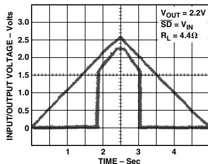
Figure 9. Power-Up/Power-Down
