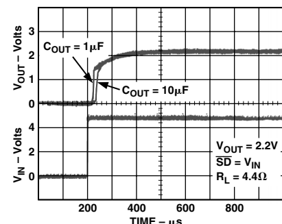
Figure 10. Power-Up Response
