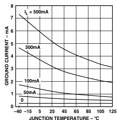
Figure 7. Ground Current vs. Junction Temperature
