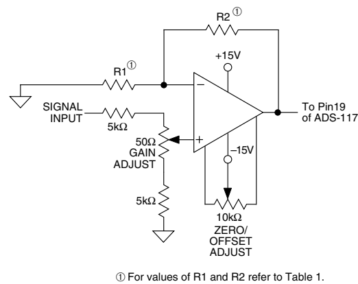
Figure 4. Optional Calibration Circuit
