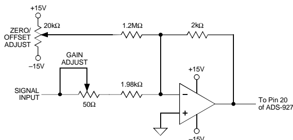
Figure 2. ADS-927 Calibration Circuit
