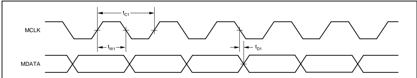
Figure 1. Mode 0 Operation
