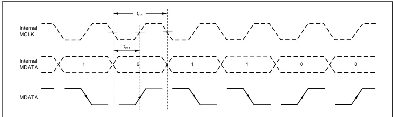
Figure 3. Mode 2 Operation
