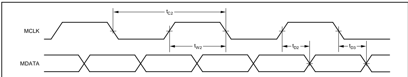
Figure 2. Mode 1 Operation
