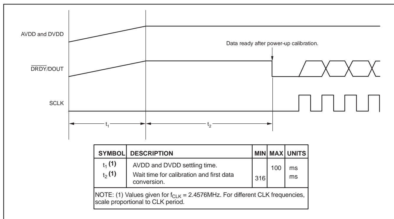
Figure 23. Power-Up Timing
