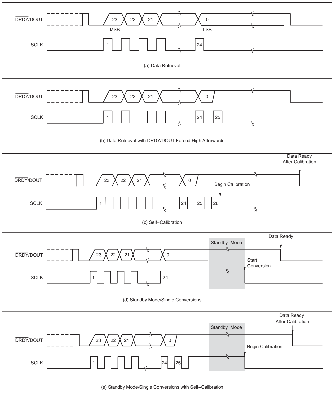
Figure 32. Summary of Serial Interface Waveforms
