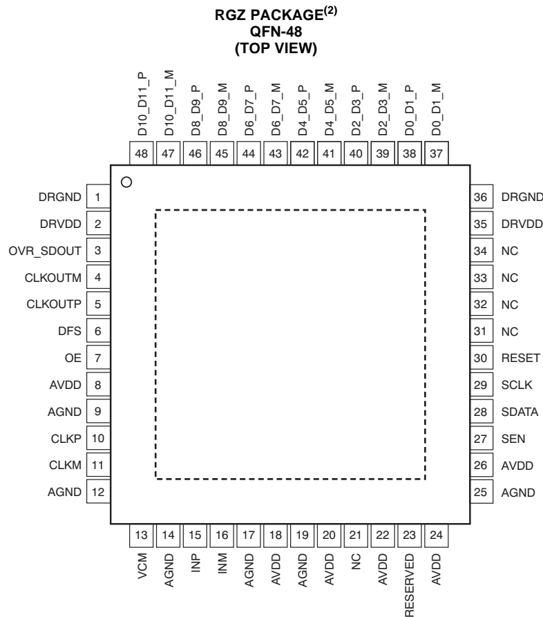
Figure 12. ADS412x LVDS Pinout (3)
