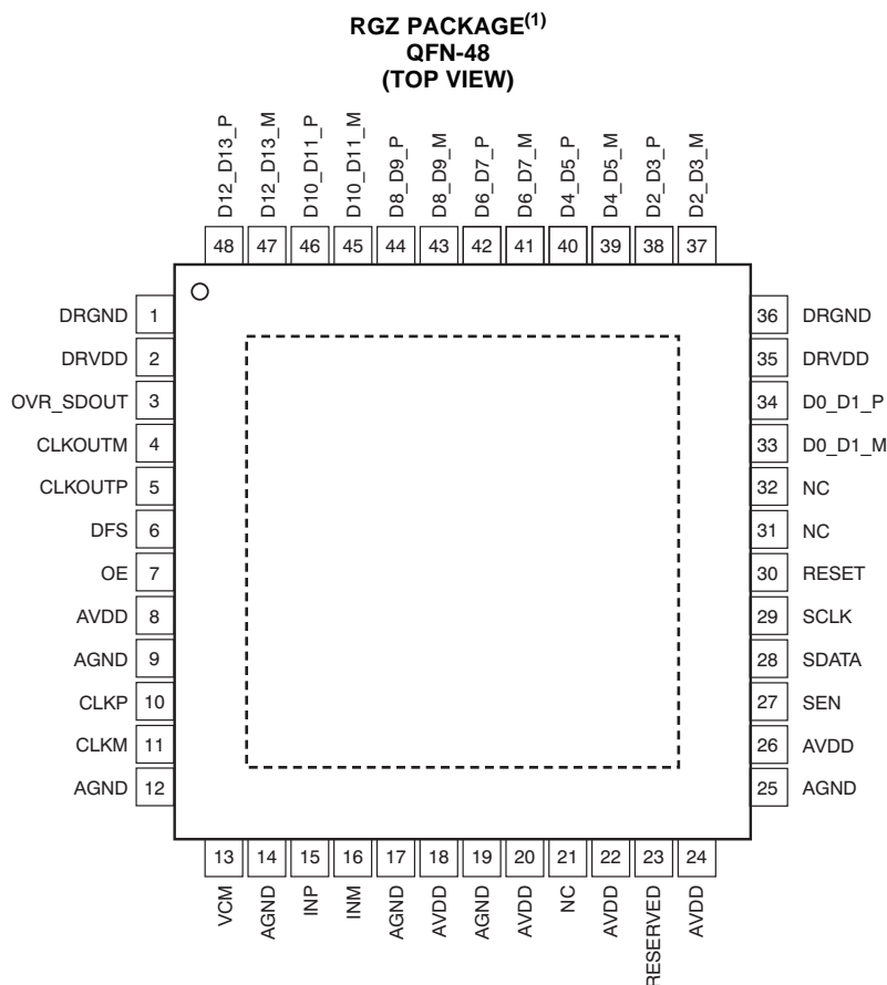
Figure 11. ADS414x LVDS Pinout
