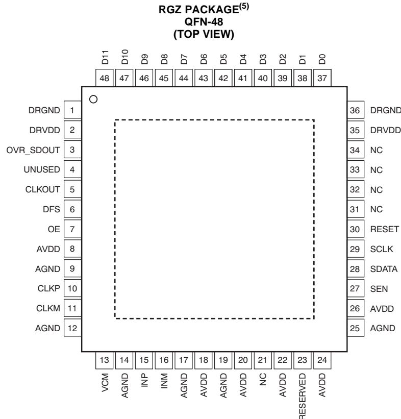
Figure 14. ADS412x CMOS Pinout (6)
