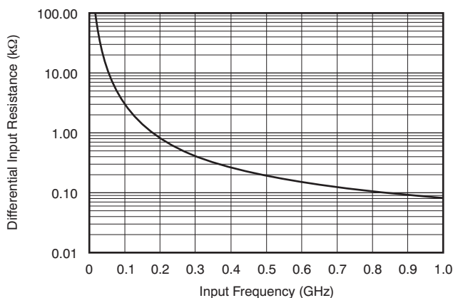
Figure 114. ADC Analog Input Resistance ( R_{IN} ) Across Frequency
