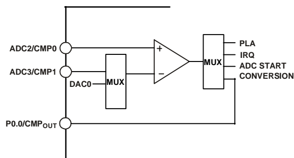
Figure 19: Comparator
