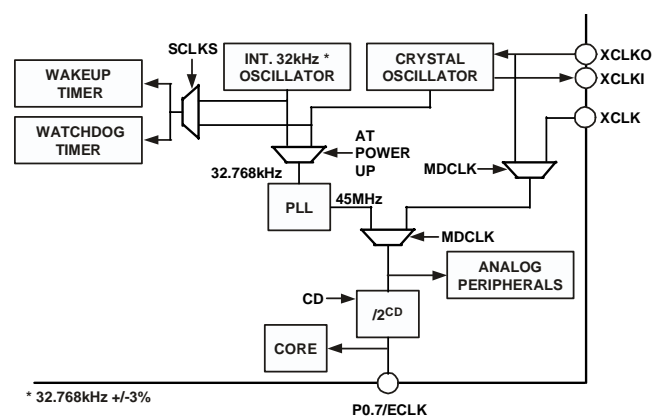
Figure 20: clocking system
