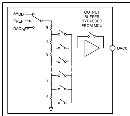
Figure 17: DAC structure
