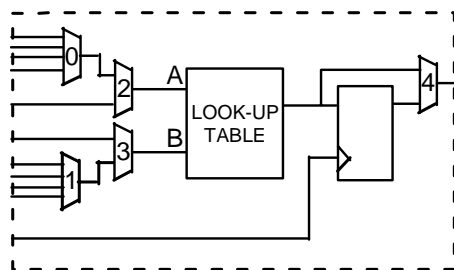
Figure 27: PLA element
