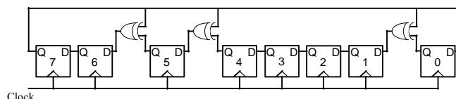
Figure 32: 8-bit LFSR
