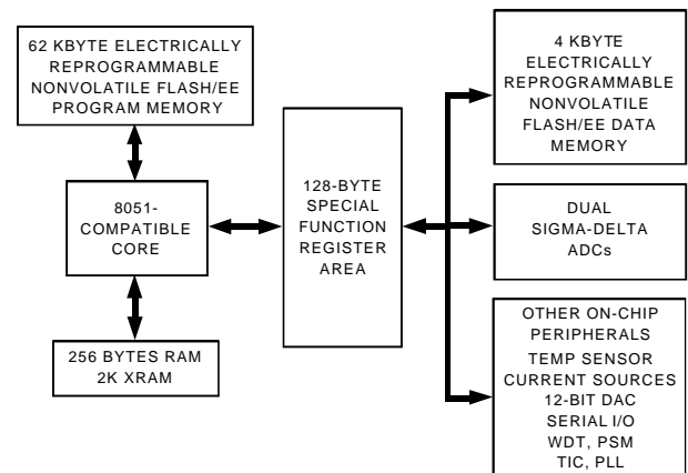
Figure 5. Programming Model
