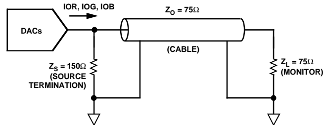
Figure 5b. Analog Output Termination for RS-170
