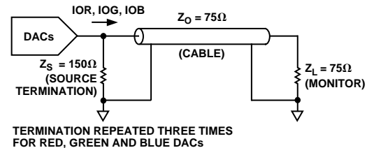
Figure 22b. Analog Output Termination for RS-170
