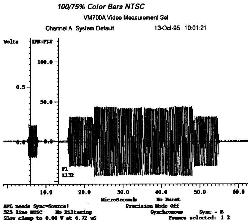
Figure 58. 100/75% Color Bars NTSC (Chrominance Only)
