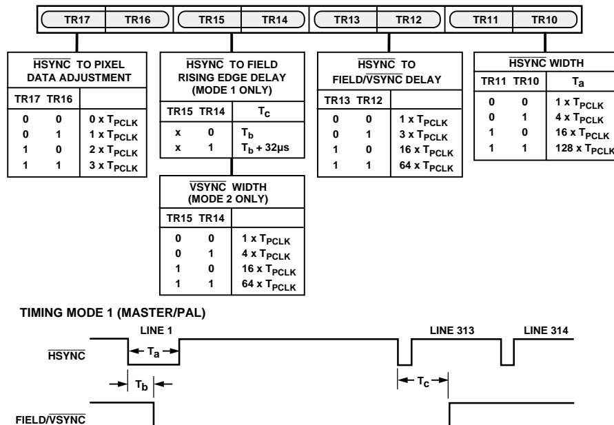
Figure 37. Timing Register 1
