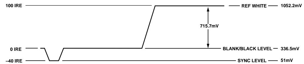
Figure 51. NTSC RGB Video Levels
