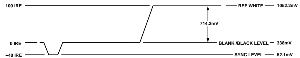
Figure 49. NTSC Luma Video Levels
