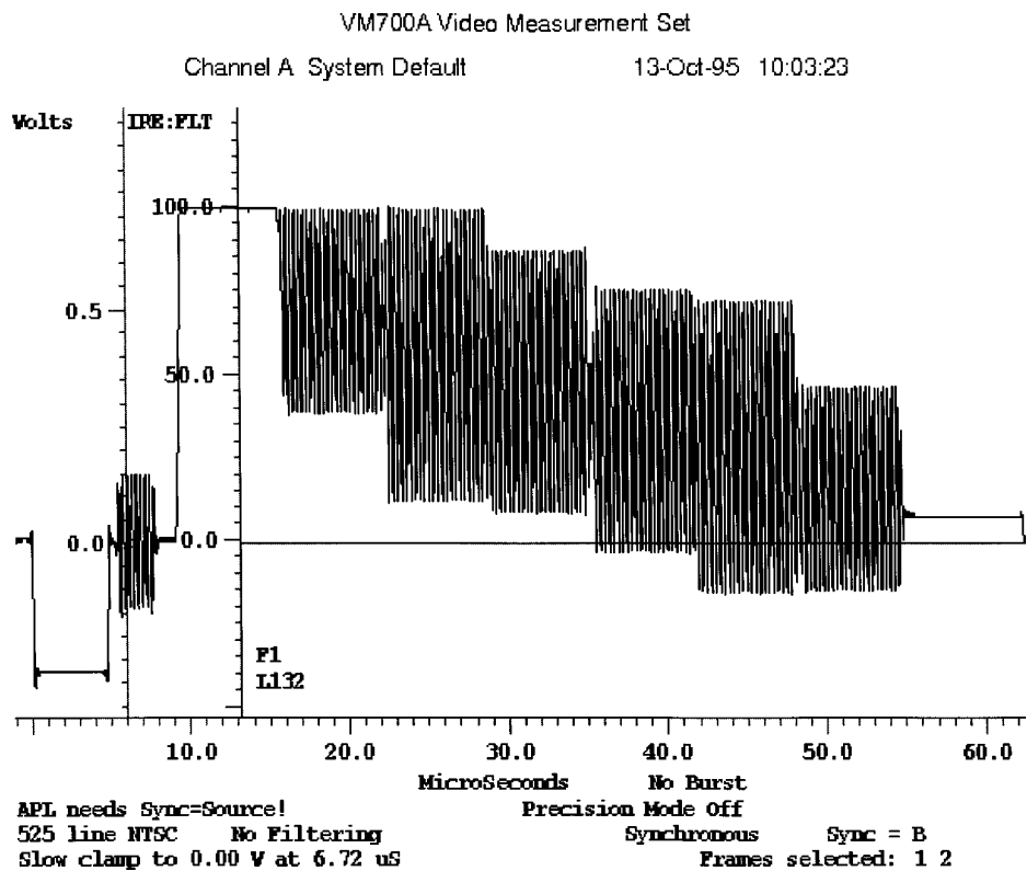
Figure 57. 100/75% Color Bars NTSC
