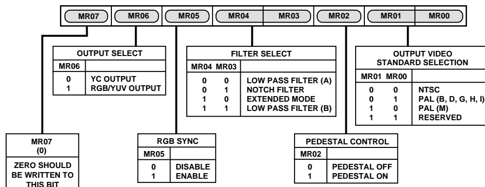
Figure 31. Mode Register 0
