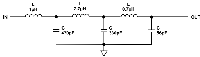
Figure 56. Output Filter
