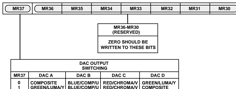
Figure 40. Mode Register 3
