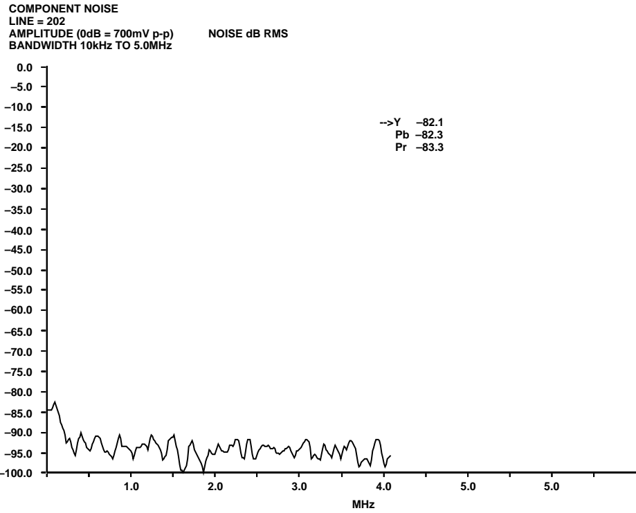
Figure 89. PAL YUV SNR Plot
