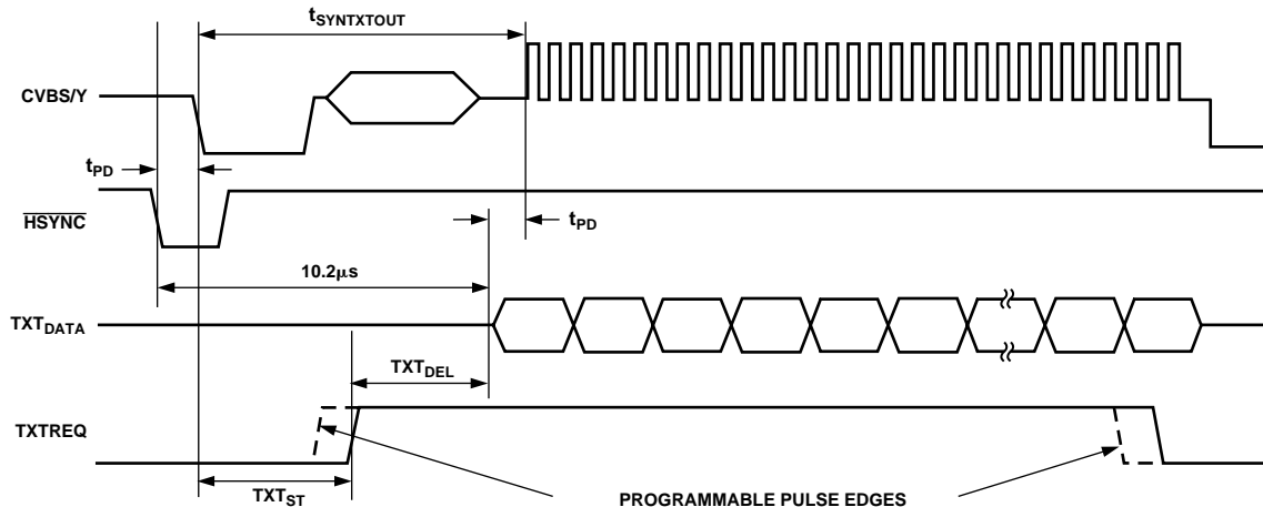
Figure 47. Teletext VBI Line
