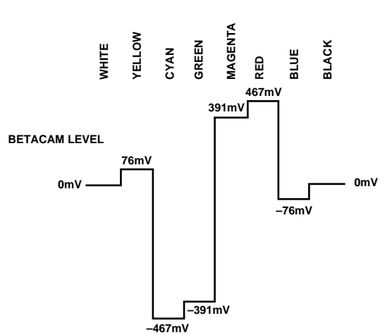
Figure 64. NTSC 100% Color Bars No Pedestal V Levels
