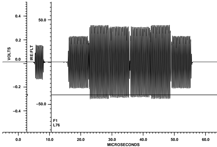
Figure 77. 100/75% NTSC Color Bars Chrominance
