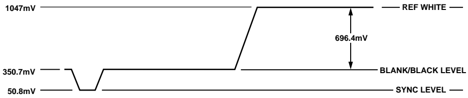
Figure 58. PAL Luma Video Levels
