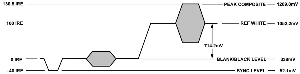
Figure 53. NTSC Composite Video Levels
