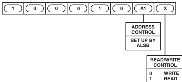
Figure 27. Slave Address
