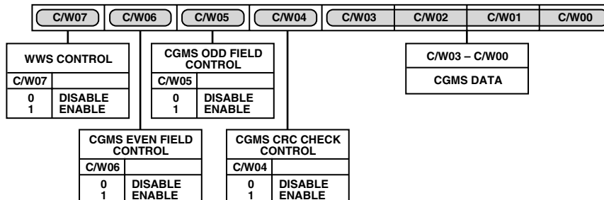
Figure 75. CGMS_WSS Register 0
