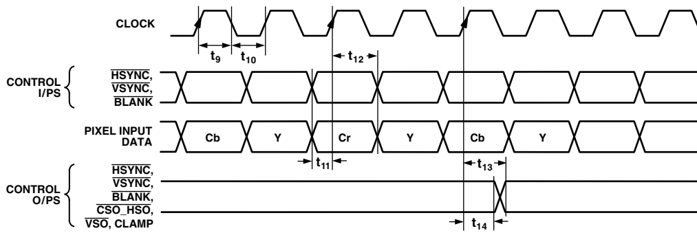
Figure 2. Pixel and Control Data Timing Diagram
