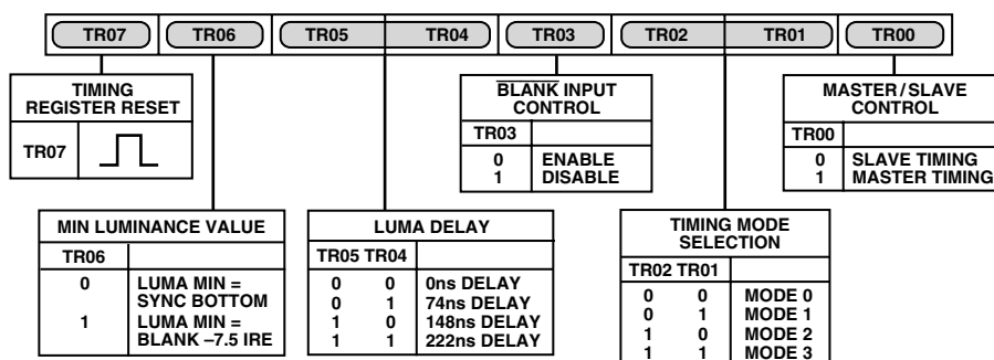
Figure 66. Timing Register 0
