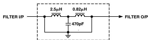
Figure 100. Output Filter for 2× Oversampling Mode
