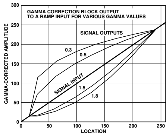
Figure 92. Signal Input (Ramp) and Selectable Gamma Output Curves
