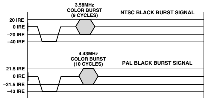
Figure 64. Black Burst Signals for PAL and NTSC Standards
