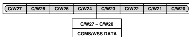
Figure 77. CGMS_WSS Register 2
