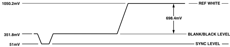
Figure 118. PAL RGB Video Levels
