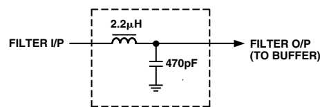
Figure 102. Output Filter for 4× Oversampling Mode
