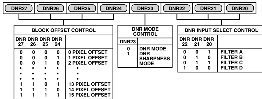
Figure 90. DNR Register 2
