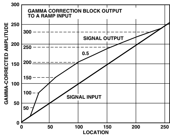
Figure 91. Signal Input (Ramp) and Signal Output for Gamma 0.5
