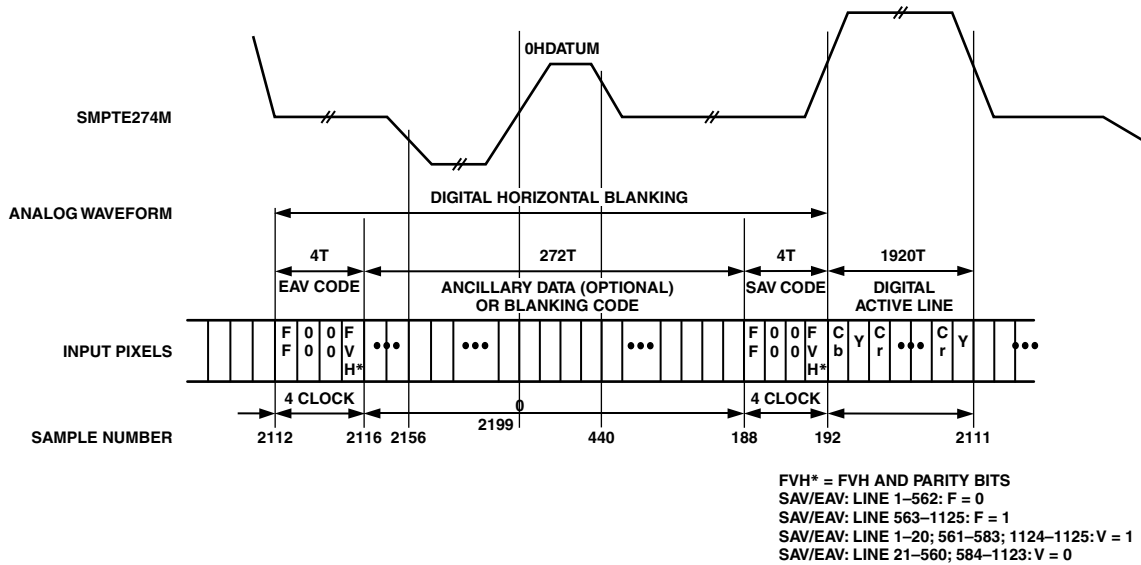
Figure 66. EAV/SAV Input Data Timing Diagram—SMPTE274M
