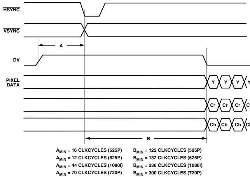
Figure 4. Input Timing Diagram
