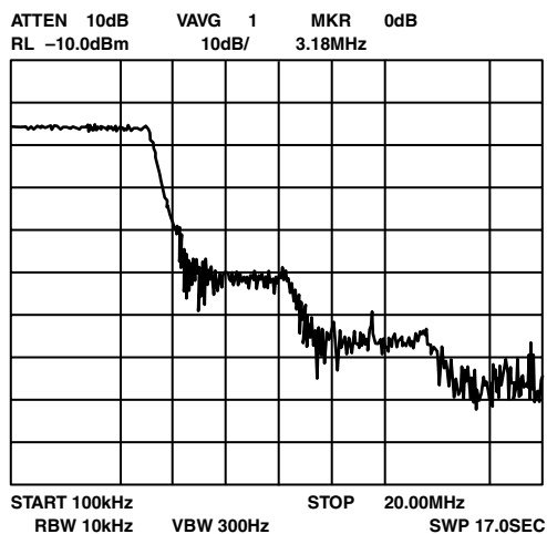
Figure 6. ADV7196A SSAF Response to a 2.5 MHz Chroma Sweep Using 4:2:2 Input Mode
