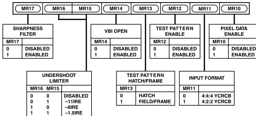
Figure 20. Mode Register 1
