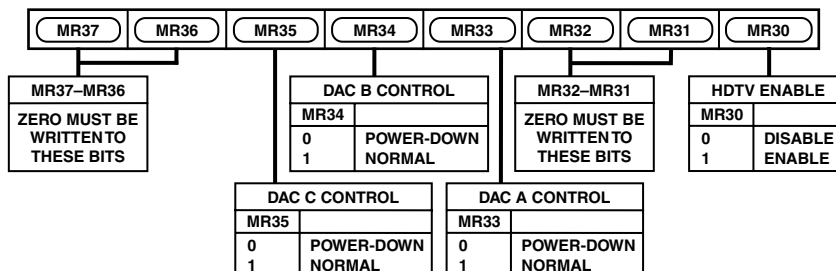
Figure 54. Mode Register 3
