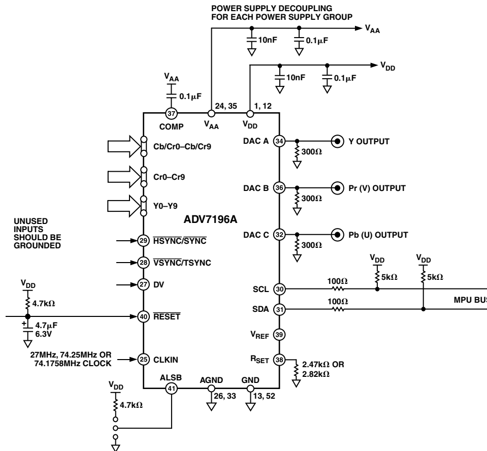
Figure 57. Circuit Layout
