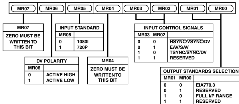
Figure 50. Mode Register 0
