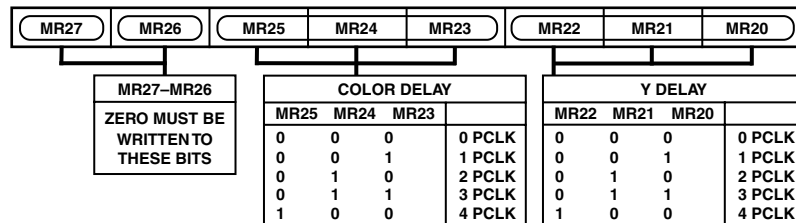
Figure 53. Mode Register 2
