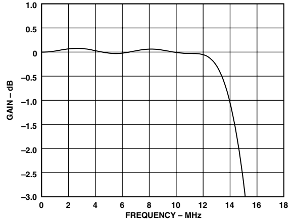
Figure 39. UV - HDTV 2× Oversampling Filter, Pass Band
