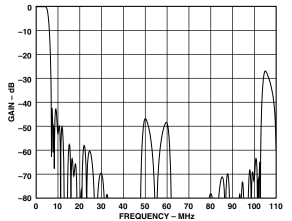
Figure 40. UV - PS 4× Oversampling Filter, SSAF
