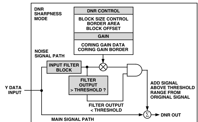
Figure 68. DNR Block Diagram
