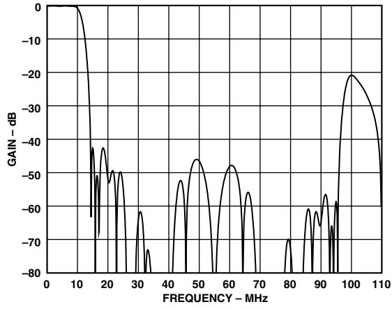
Figure 37. UV - HDTV 2× Oversampling Filter
