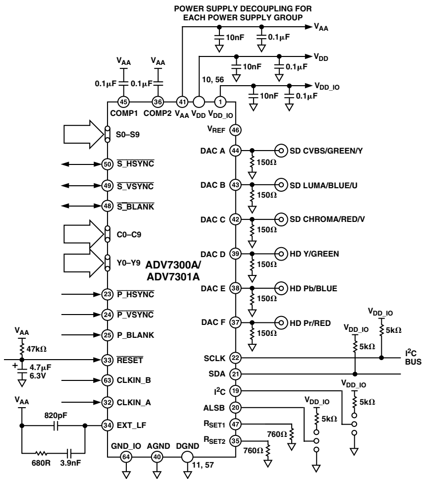
Figure 79. Circuit Layout
