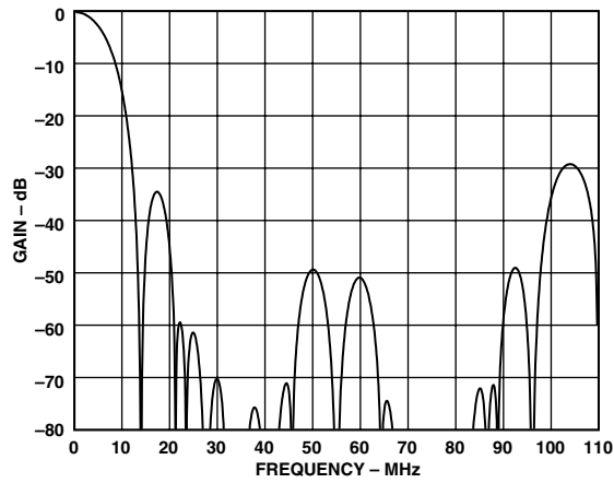
Figure 38. UV - PS 4× Oversampling Filter, Linear
