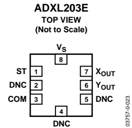
Figure 23. ADXL203 8-Lead CLCC
