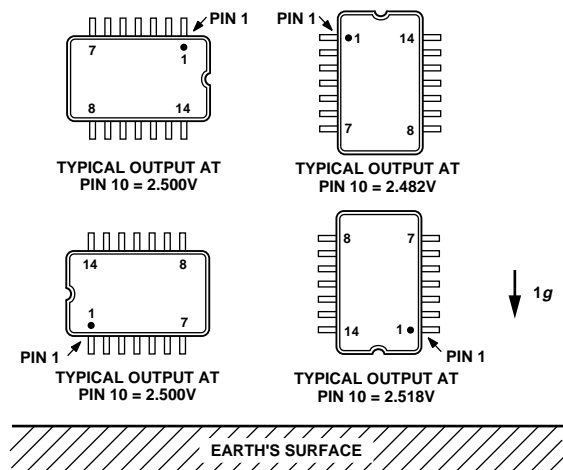
Figure 1. ADXL190 Response Due to Gravity
