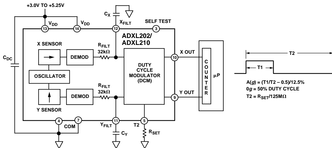
Figure 13. Block Diagram
