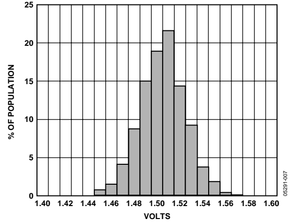
Figure 7. Y-Axis Zero g Bias at 25°C
