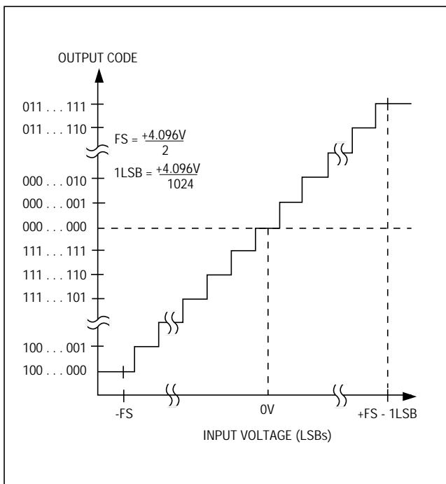
Figure 16. Bipolar Transfer Function, \pm 4.096\text{V}/2 = \text{Full Scale}
