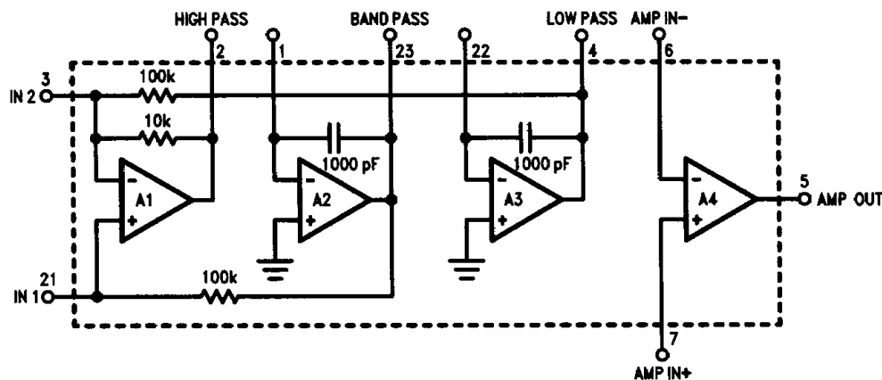
FIGURE 1. AF151 Schematic (Section 1)
