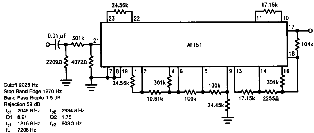
FIGURE 12. High Pass Low Speed Asynchronous FSK Modem Filter
