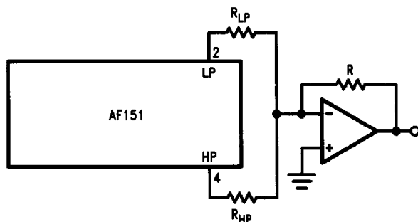
FIGURE 7. Notch Filter
