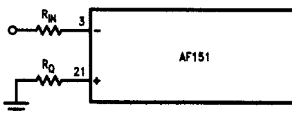
FIGURE 6. Connection for Any Q, Inverting
