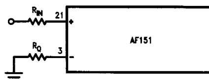
FIGURE 5. Connection for Q < Q_{MIN}
