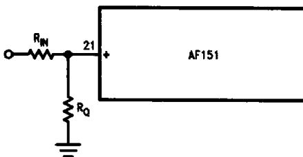
FIGURE 4. Connection for Q > Q_{MIN}
