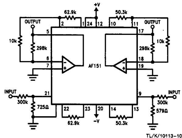
FIGURE 8. Dual Band Pass Filter
