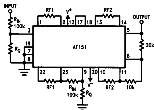
FIGURE 9. Telephone Multifrequency (MF) Band Pass Filter
