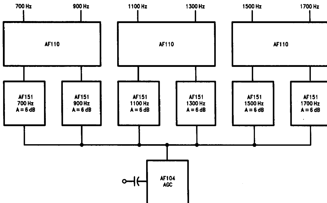
FIGURE 10. MF Tone Receiver
