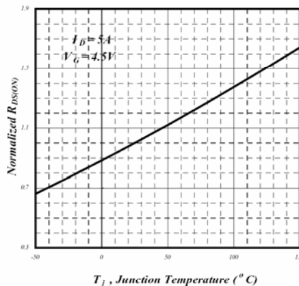
Fig 4. Normalized On-Resistance
