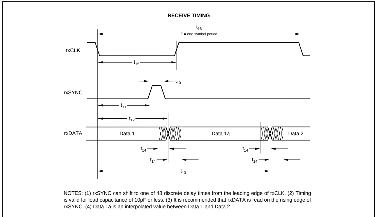
FIGURE 5. Receive Timing Diagram.
