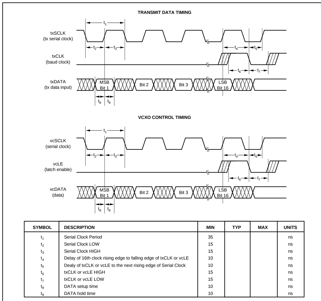
FIGURE 4. Timing Diagram.
