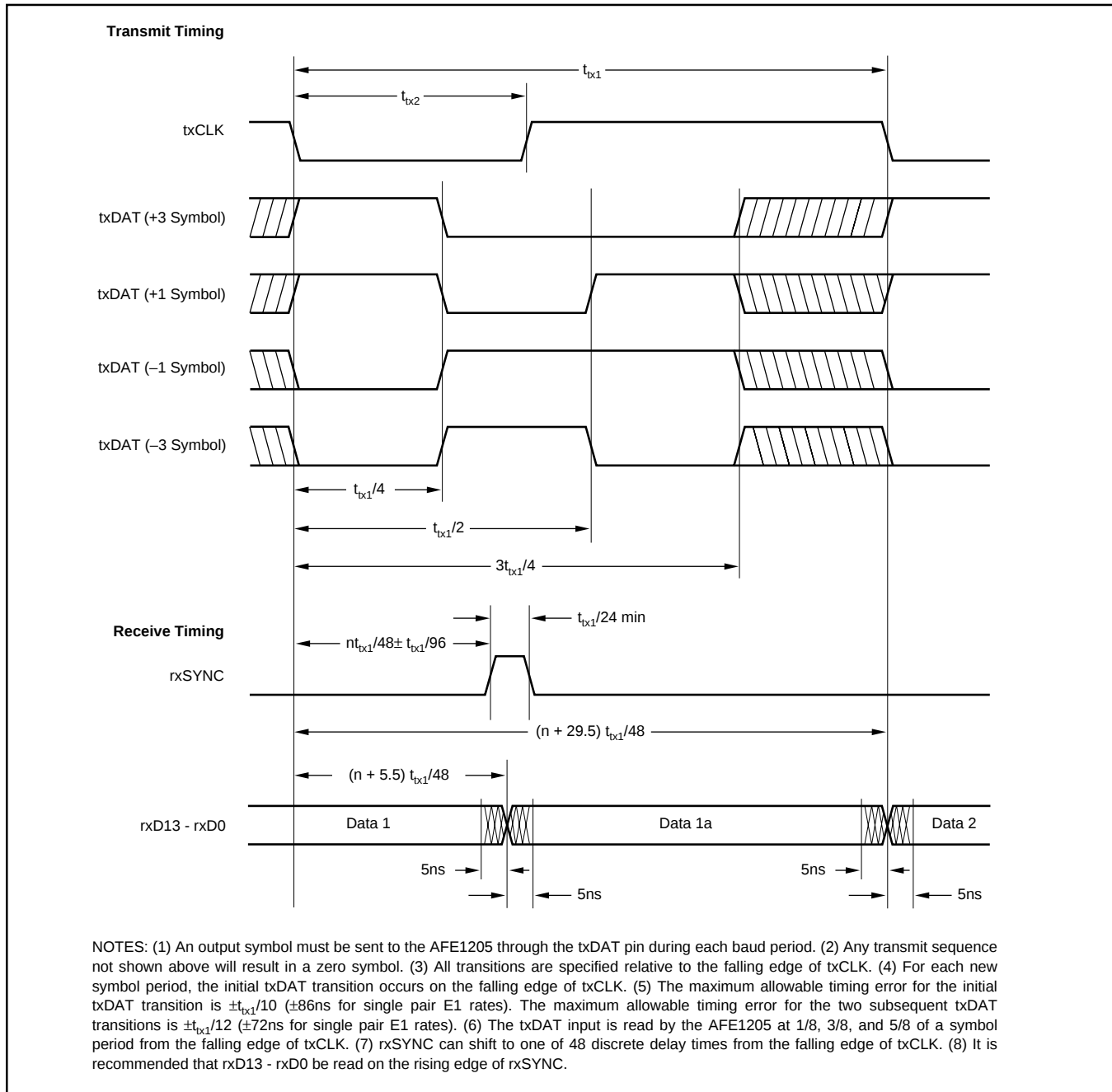
FIGURE 3. Timing Diagram.
