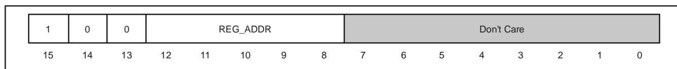
Figure 5. Register Write Instruction Format
