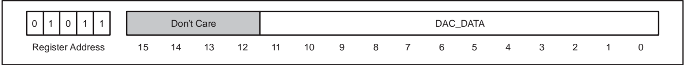
Figure 19. Auxiliary DAC Control Register
