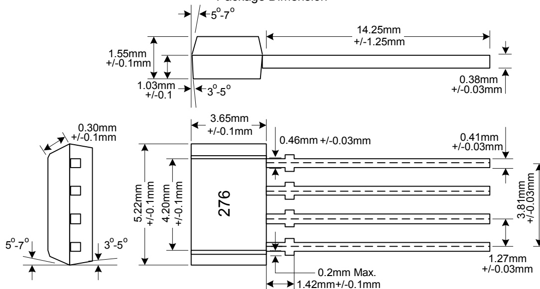
Package Dimension
