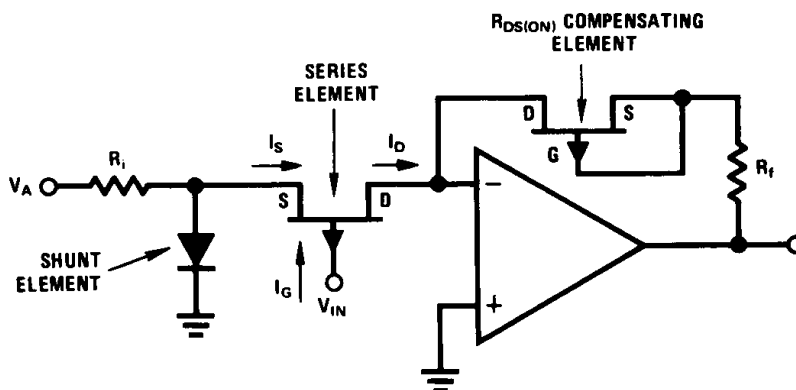
FIGURE 6. Definition of Terms
