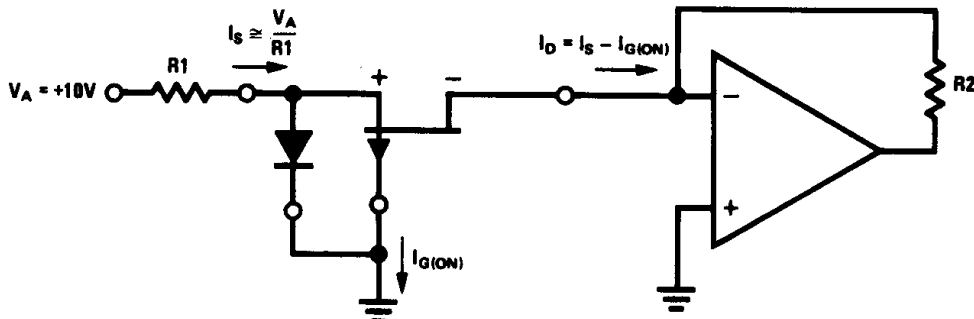
FIGURE 2. On Leakage Current, I_{G(ON)}
