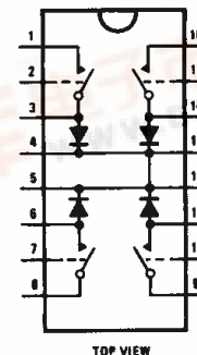
Dual-In-Line Package
