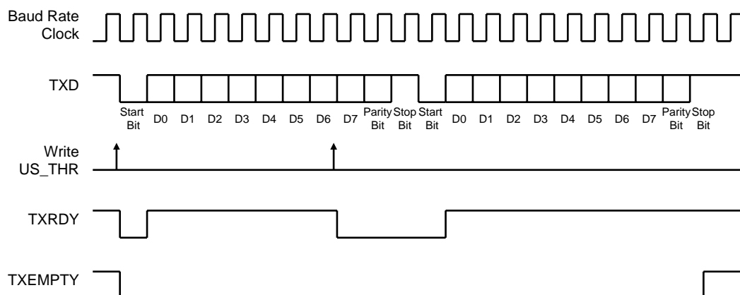
Figure 95. Transmitter Status
