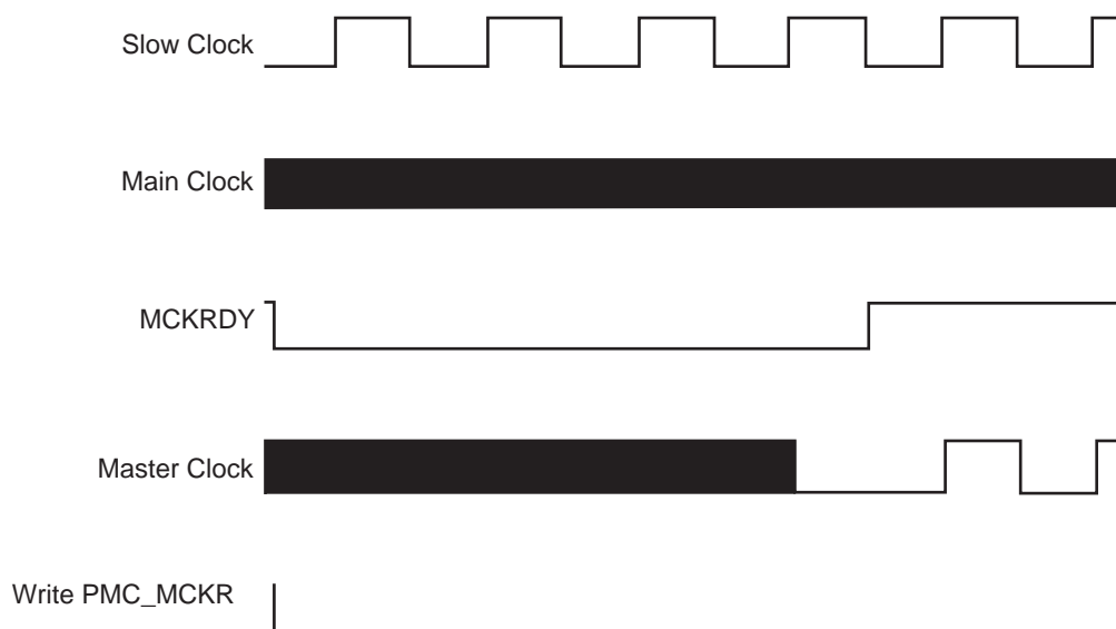
Figure 44. Switch Master Clock from Main Clock to Slow Clock
