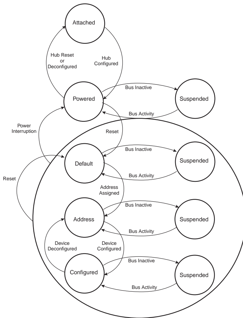
Figure 176. USB Device State Diagram
