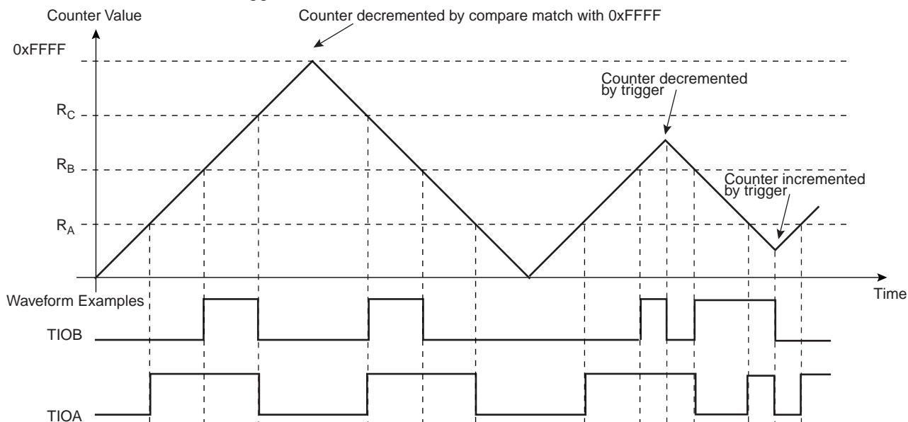
Figure 148. WAVSEL = 01 With Trigger
