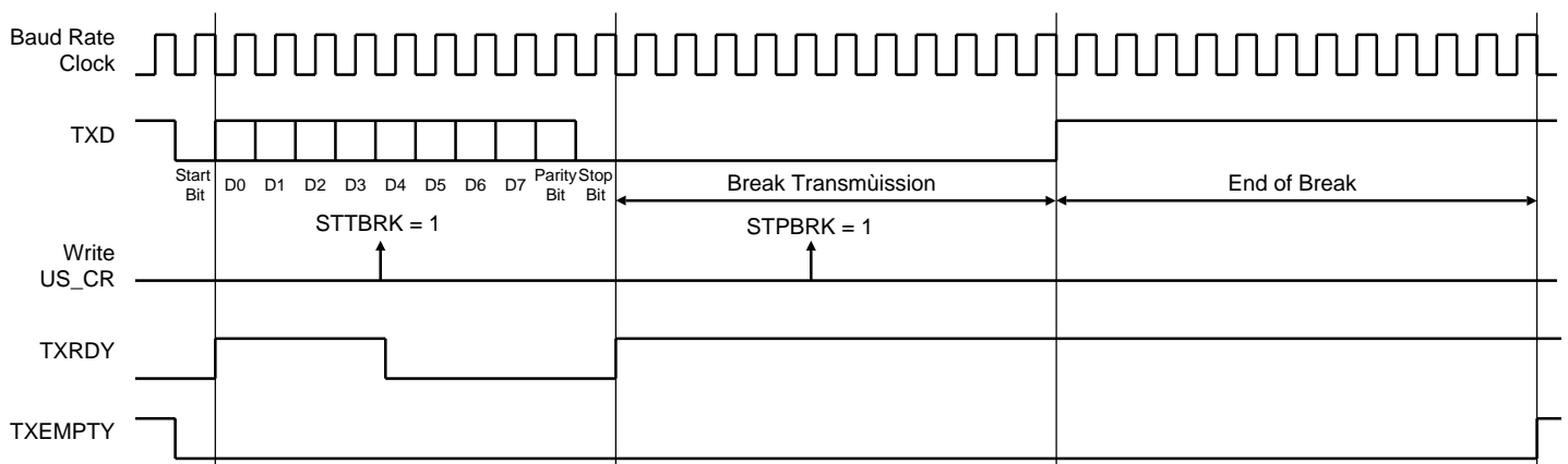
Figure 104. Break Transmission
