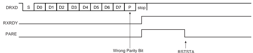
Figure 60. Parity Error
