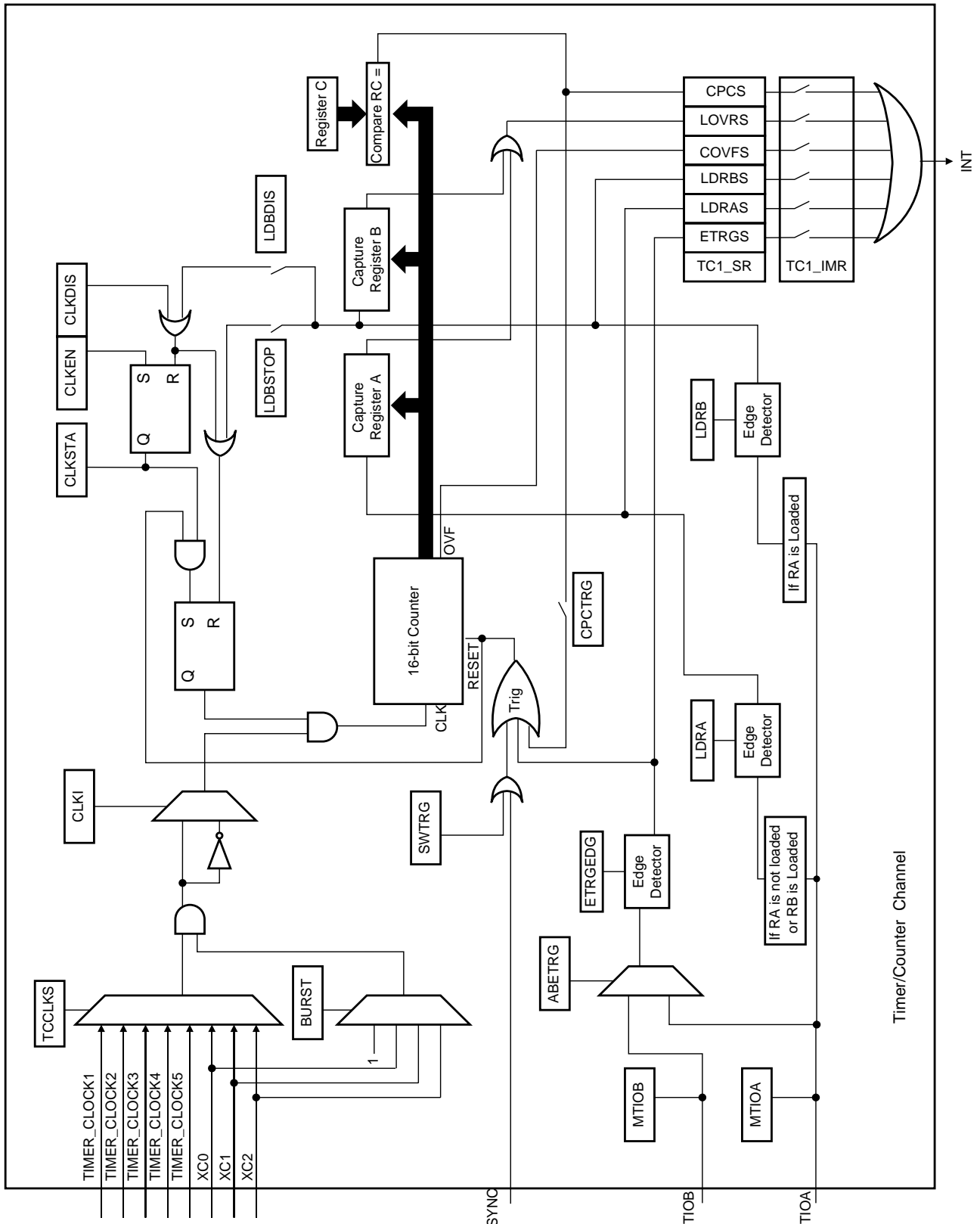
Figure 141. Capture Mode
