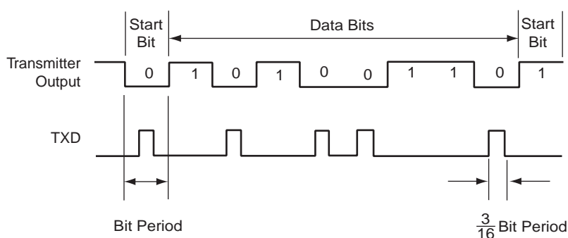
Figure 112. IrDA Modulation
