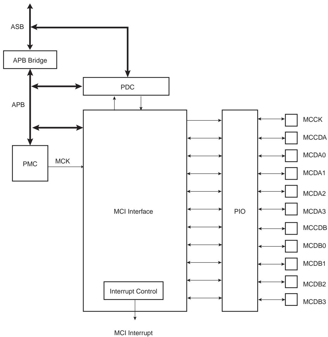
Figure 151. Block Diagram
