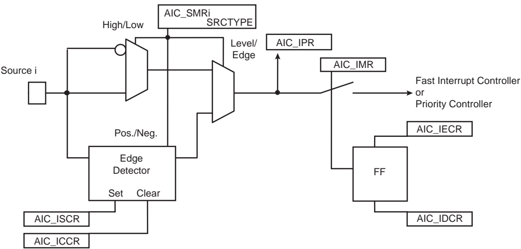
Figure 29. External Interrupt Source Input Stage
