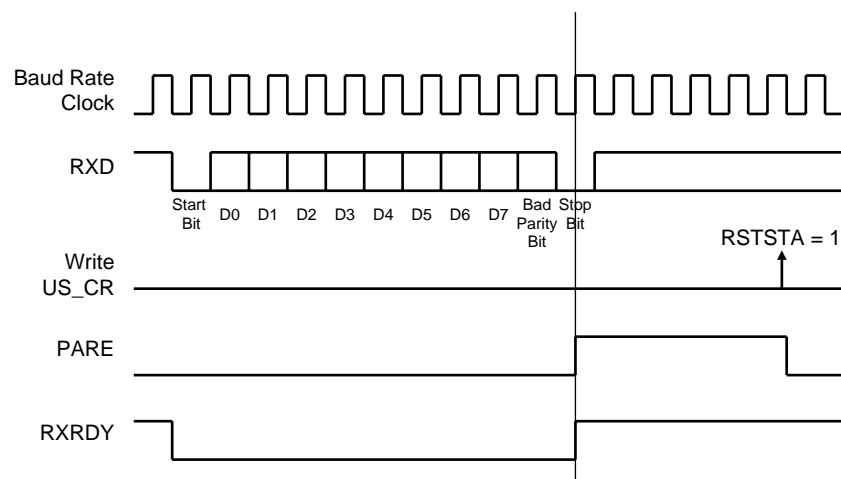
Figure 100. Parity Error
