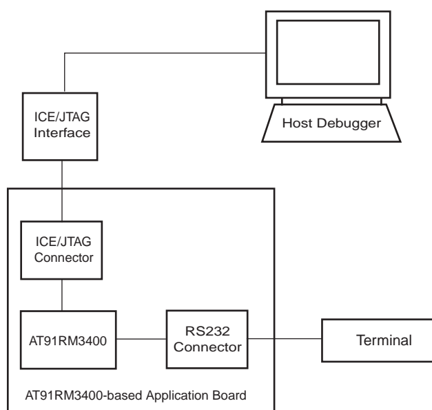
Figure 7. AT91RM3400-based Application Debug Environment Example
