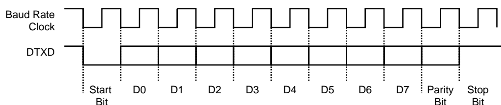
Figure 62. Character Transmission
