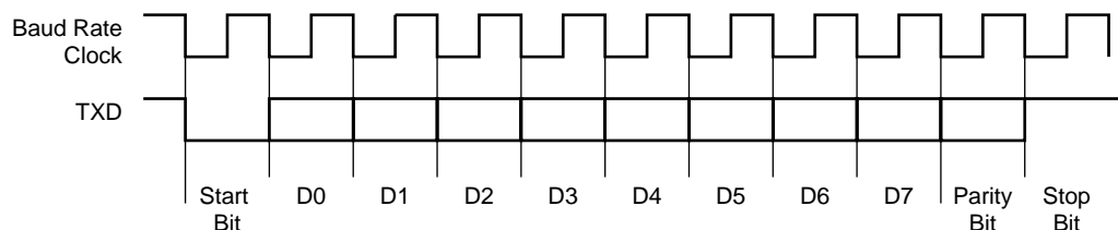
Figure 94. Character Transmit
