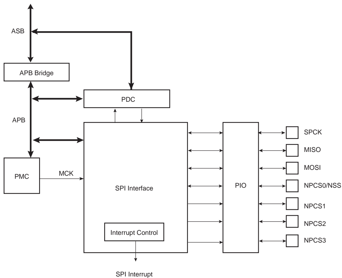
Figure 71. Block Diagram
