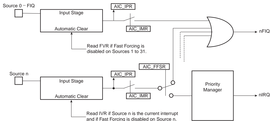
Figure 34. Fast Forcing
