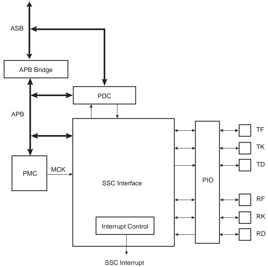
Figure 120. Block Diagram
