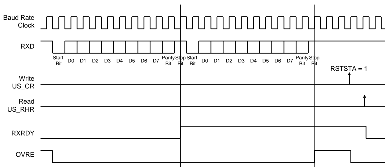
Figure 99. Receiver Status
