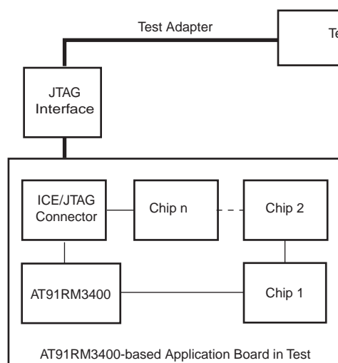
Figure 8. AT91RM3400-based Application Test Environment Example
