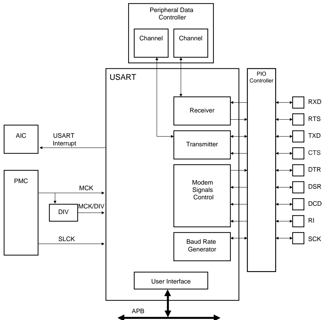
Figure 90. USART Block Diagram
