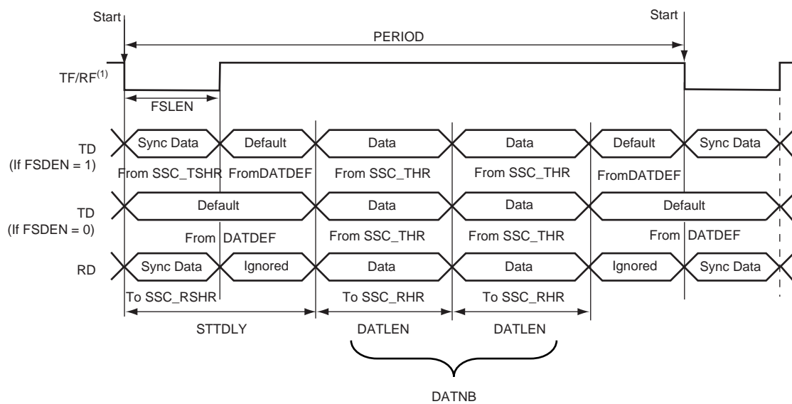
Figure 131. Transmit and Receive Frame Format in Edge/Pulse Start Modes
