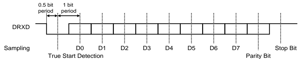
Figure 57. Character Reception
