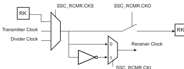
Figure 126. Receiver Clock Management
