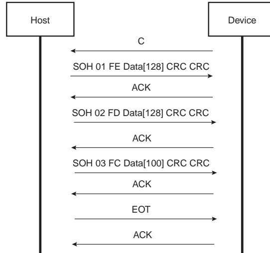
Figure 17. Xmodem Transfer Example
