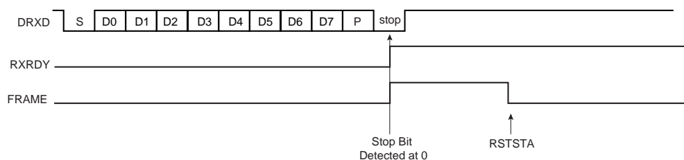
Figure 61. Receiver Framing Error
